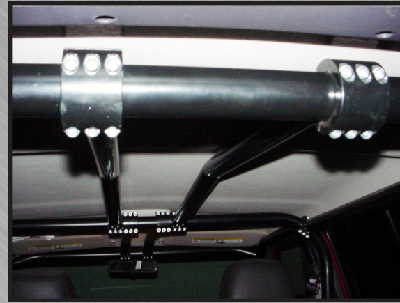
XJ REAR CENTER BAR UNPAINTED $99.95 EACH BAR
