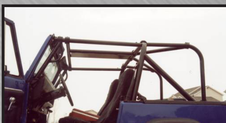
YJ REAR SIDE & ANGLE BARS 1987-91 PART # RH1002-C $329.95 *DESIGNED TO BE USED WITH FRONT CAGE KIT. ADDITIONAL CLAMPS (PART #RH1001-G) ARE NECESSARY IF USING ALONE.
