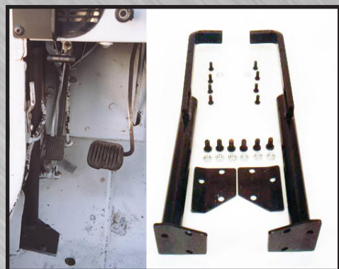
CJ7 FLOOR MOUNTS 1976-1986 PART # RH1003-F $169.95
