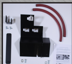
CANISTER RELOCATION KIT PART# RH 6005-A (2007-2011) PART# RH 6005-B (2012-2015) $119.95
