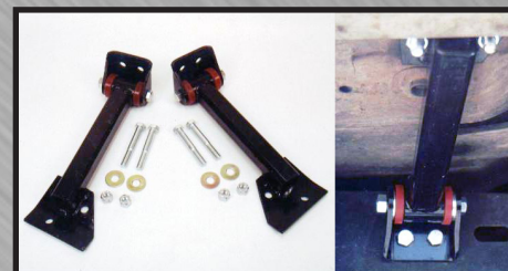
YJ FRAME MOUNTS UNPAINTED 1987-1995 PART # RH1002-G $109.95
