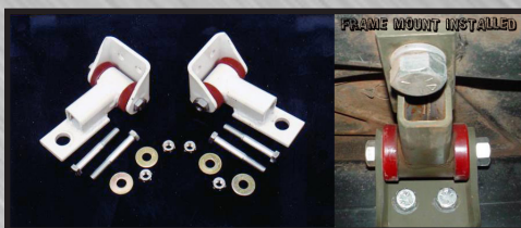
TJ & LJ FRAME MOUNTS UNPAINTED 1997-2006 PART # RH1001-E $109.95
