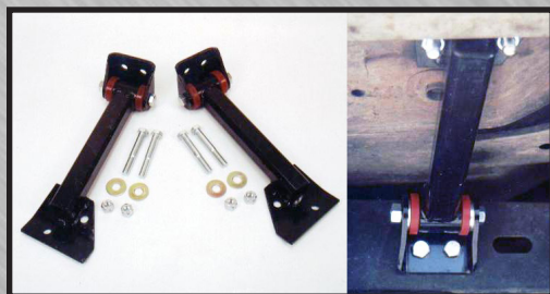
CJ5 FRAME MOUNTS UNPAINTED 1976-1983 PART # RH1003-G $109.95
